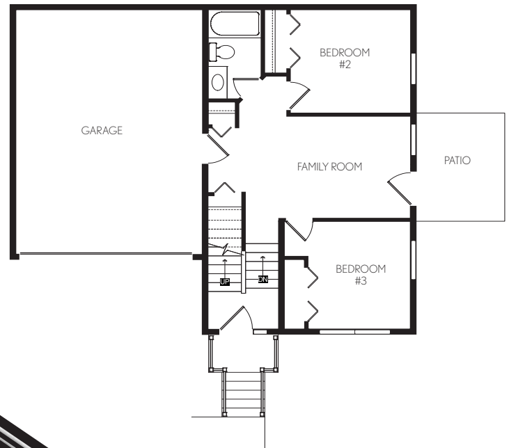
Optional Lower Level with Third Bedroom
